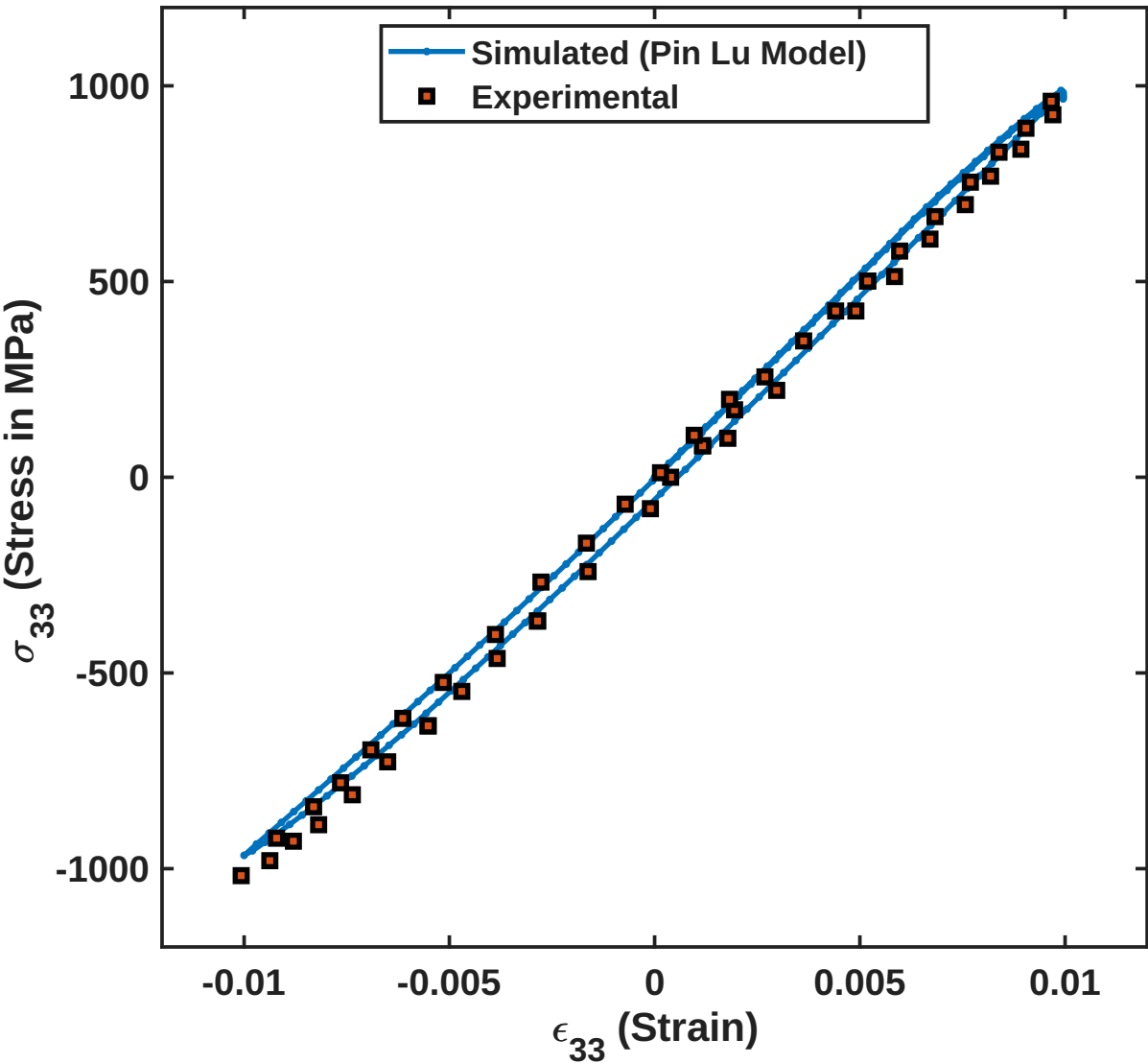
Fatigue Test: Simulated vs Experimental
